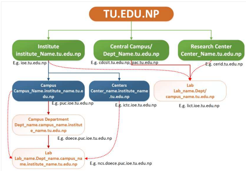
Figure 2 DNS Hierarchy of TU
